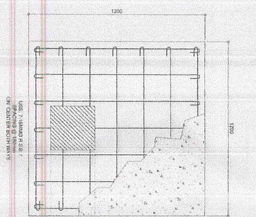
FOOTING & COLUMN DETAIL SCALE 1:10
